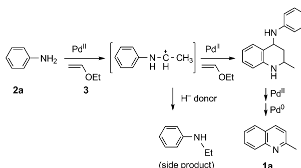
Scheme 1. Formation of 2-methylquinoline ( 1a ) from aniline ( 2a ) and ethyl vinyl ether ( 3 ).
